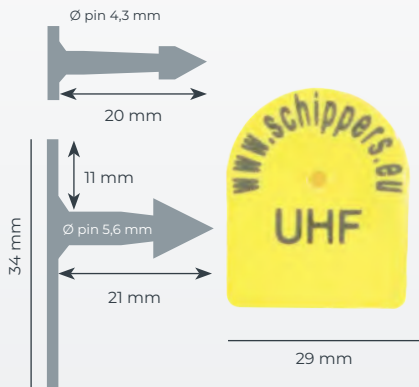
MS Tag Torbogen UHF
