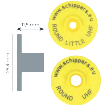
MS Tag Round UHF (Open)
