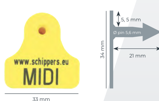
MS Tag Midi (Plastic pin)
